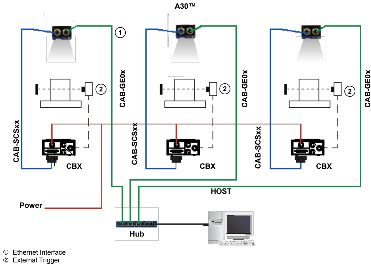
Figure 46 - Ethernet Network Layout
